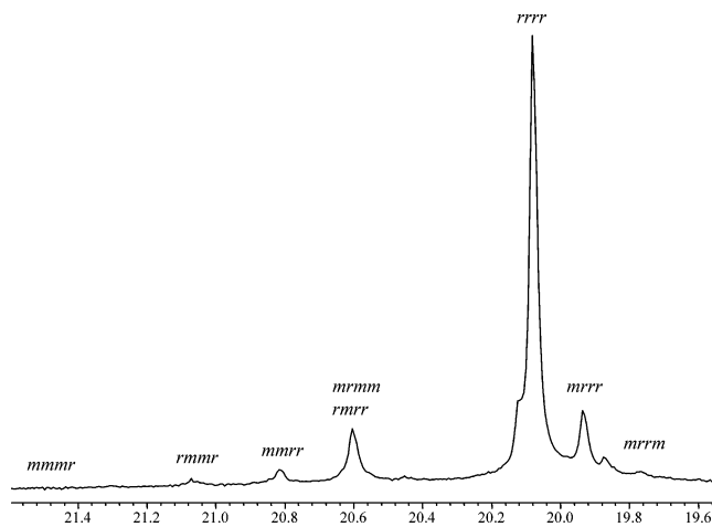
Figure 7. ^{13}\text{C} NMR spectrum (125.72 MHz) of polypropylene made with catalyst 8a /MAO.
